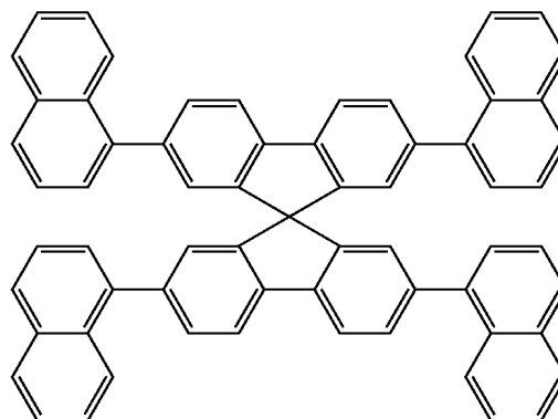
Structural formula (5)
